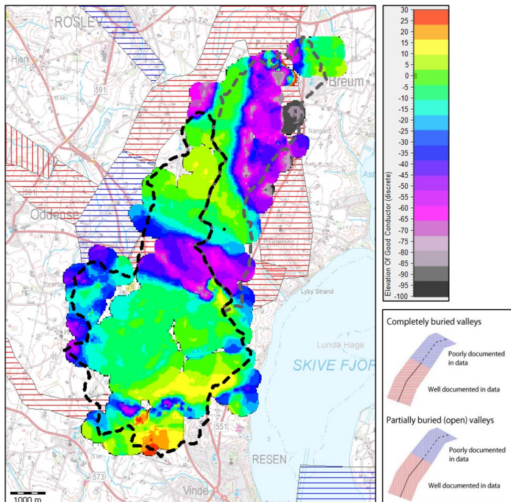
Figure 6.17: Elevation of good conductor in tTEM data. The criterion is that the deep low-resistive layer in the smooth tTEM models must be < 10 Ohmm. Red and blue shaded polygons represent mapped buried valleys (see Figure 6.7; Sandersen & Jørgensen, 2016).
